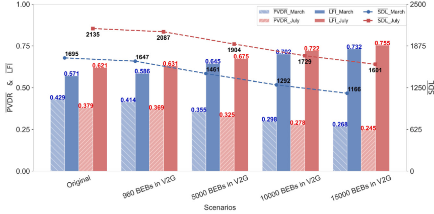
(b) the peak-shaving performance measurement
